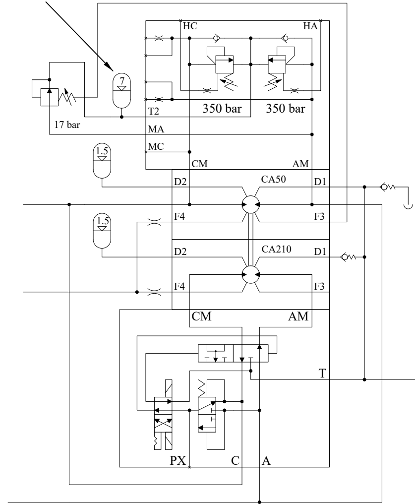
Charge Pressure Accumulator
